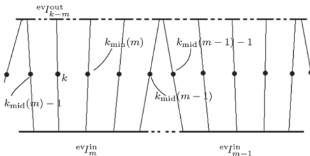
Figure 15. The curves {}^{\text{ev}}\gamma_k starting at {}^{\text{ev}}I_m^{\text{in}} and {}^{\text{ev}}I_{m-1}^{\text{in}} for fixed m . Exactly for k_{\text{min}}(m) \leq k \leq k_{\text{mid}}(m) - 1 , the curves \text{odd}\tilde{\gamma}_k have the same behaviour as {}^{\text{ev}}\gamma_k .
